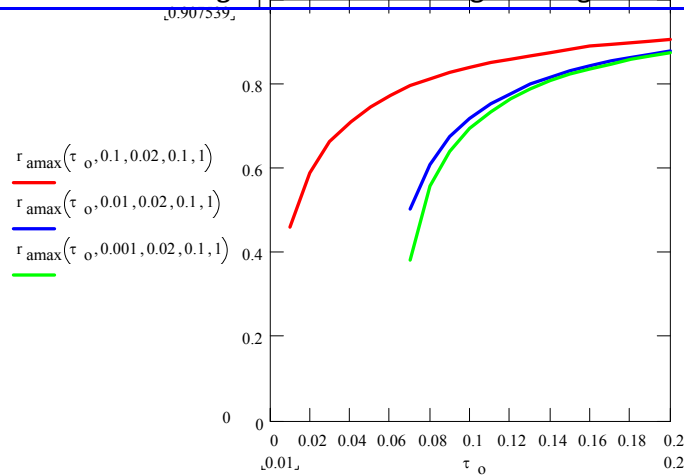
Fig.7 Solutions of the existence condition r_{a \max}(\tau_0, \beta, k_{ad}, k_{as}, \alpha)
