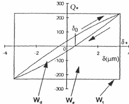
Fig.1.Representation of the various parameters characterising the fretting cycle under partial slip condition
