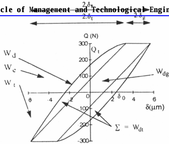
Fig.2.Representation of the various parameters characterising the fretting cycle under gross conditions
