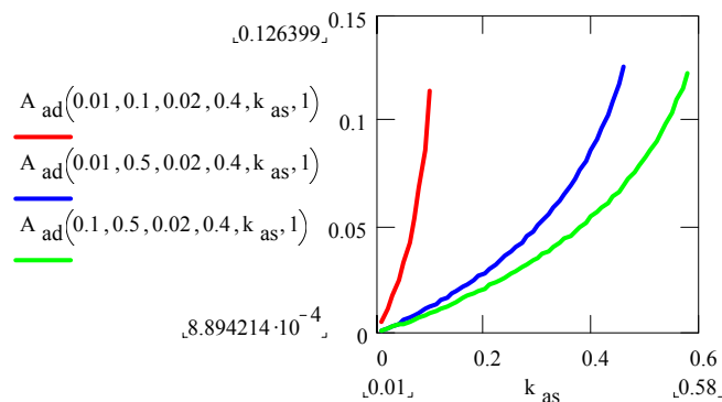
Fig.8 The dependence of the energetical ratio A_{ad}(\tau_0, \beta, k_{ad}, r_a, k_{as}, \alpha)
