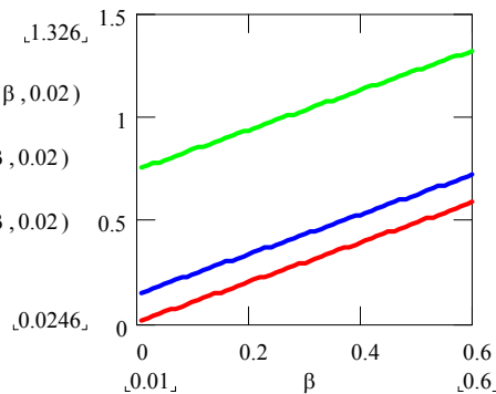
Fig.5. Solutions of the existence condition: k_{asse}(\tau_0, \beta, k_{ad})
