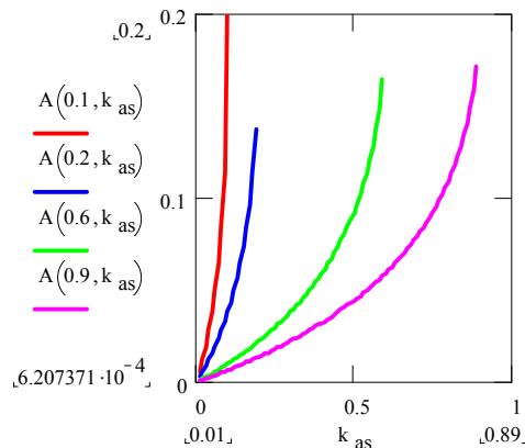
Fig.3.The variation by the energy ratio A
